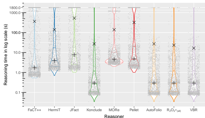
Figure 1. Reasoning time comparison between component reasoners and meta-reasoners from R_2O_2^* [9].
